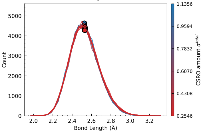
Co-Co Bond Length Distribution
